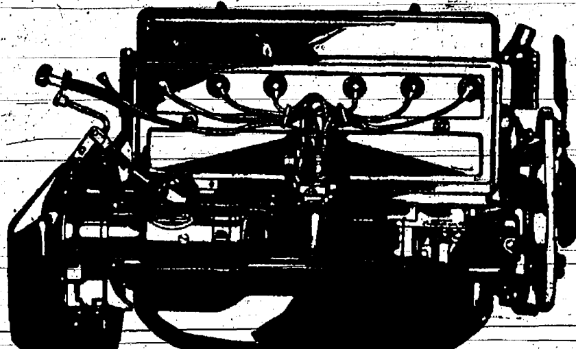
Chevrolet's new six-cylinder, fully enclosed valve-in-head engine has a high compression non-defeating head. Its piston displacement is 194 cu. in. and it develops 48 h.p. at low engine speed.
